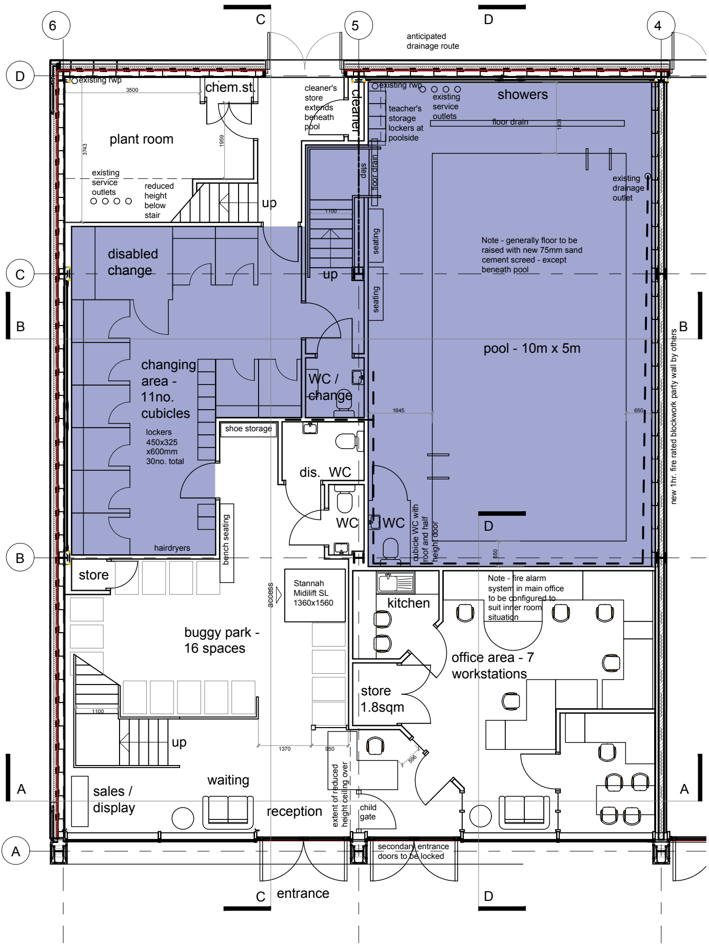
01 Proposed Ground Floor Plan 11 Scale 1:100 @ A3
